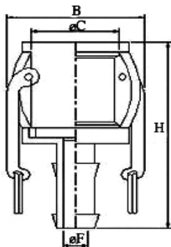
Type C Hose Shank Coupler
